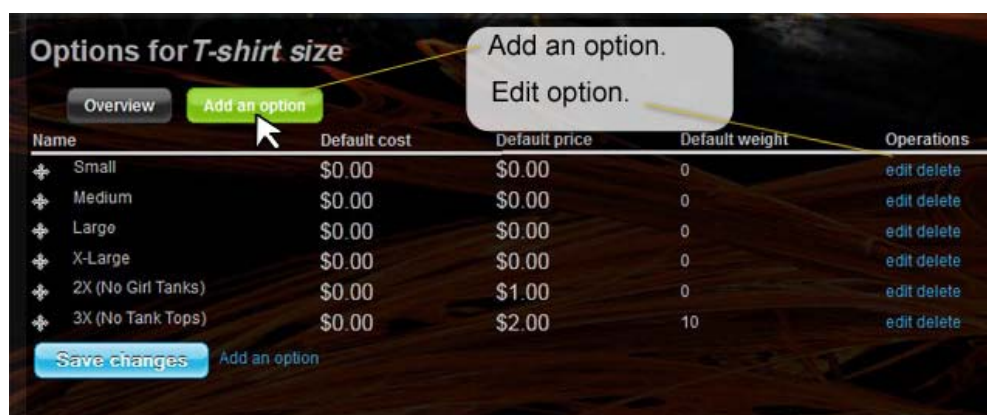
Options list, editing and reordering page.
